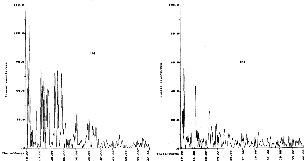
Fig. 6. (a) XRD-patterns of [Ni(ibn) 3 ]C 4 O 4 ( 10a ) [values of 2\theta and d for major lines: 10.858, 8.1419; 11.479, 7.7027; 16.098, 5.5014; 16.669, 5.3141; 17.300, 5.1218; 18.220, 4.8651; 18.900, 4.6916; 21.808, 4.0722; 22.923, 3.8764; 24.511, 3.6289.]. (b) XRD-patterns of [Ni(ibn) 3 ]C 4 O 4 ( 10b ) [values of 2\theta and d for major lines: 10.787, 8.1949; 11.419, 7.7430; 16.108, 5.4981; 21.823, 4.0694; 24.482, 3.6330.].
